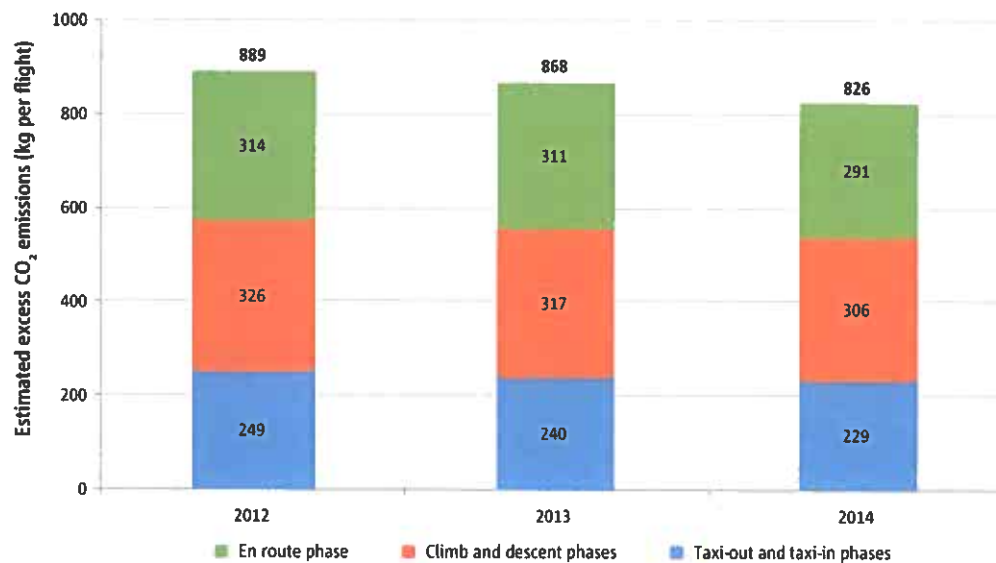
Figure 4.4 Estimated excess CO 2 emissions per flight are decreasing in taxi, take-off, climb/descent and en route phases 26
