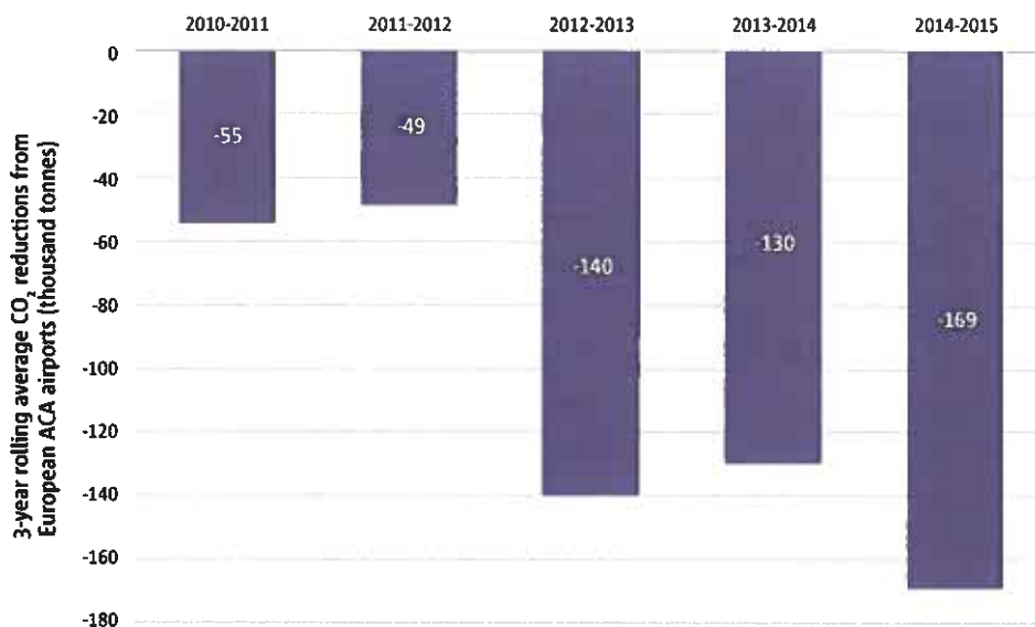
Figure 5.2 Absolute reductions 35 in airport CO 2 emissions every year since 2010
